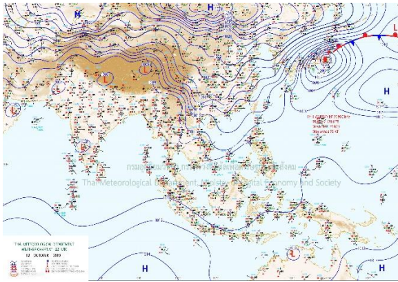
Figure 1: Weather map for 12 th Oct 2019
