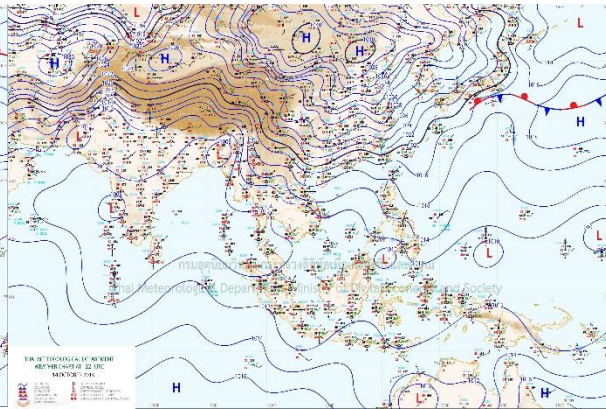
Figure 2: Weather map for 14 th Oct 2019
