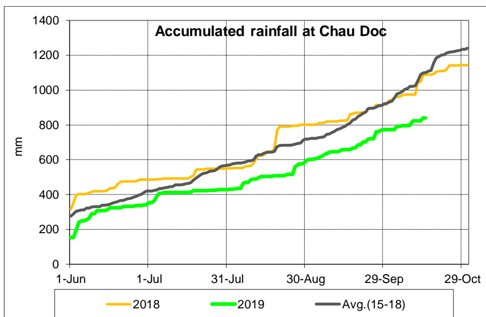
Figure 4: Accumulated Rainfall up to 15 th October to 2019 in specific stations over the LMB
